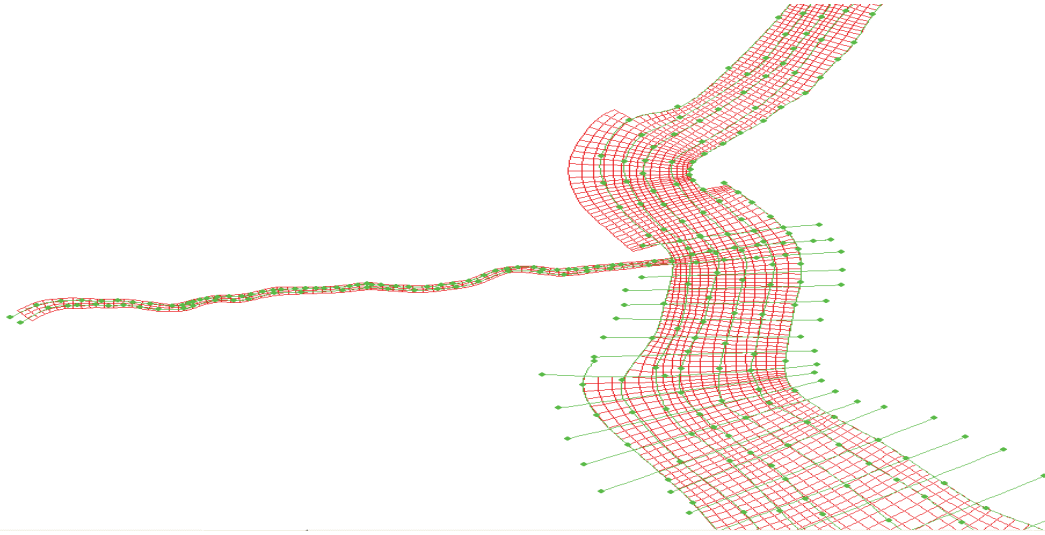
Figure 5.1. Map depicting Delaware River and Bay DELFT-3D High Resolution Grid in the C&D Canal Region. Splines are constructed through the appropriate points along each coordinate direction. Within each rectangle formed by the intersection of the splines, the number of grid cells in each coordinate direction is specified.
