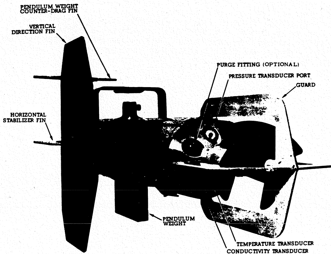
Figure 3.—Grundy 9021 G Current Meter
