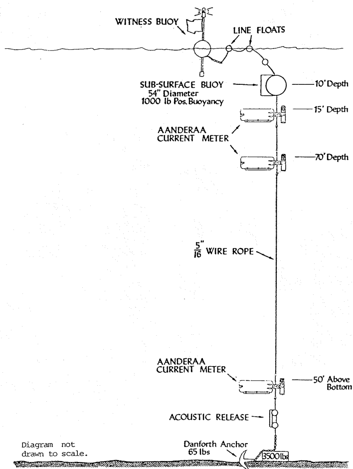
Figure 14.--Aanderaa current meter (Model RCM4) used during Puget Sound Approaches Circulatory Survey.
